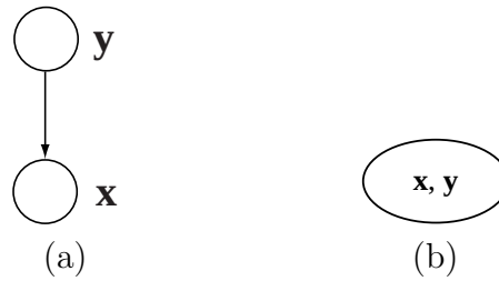
Figure 5-9: A factor analyzer as a hybrid Bayesian network and its (trivial) clique tree.
