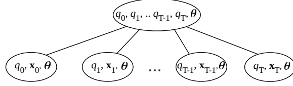
Figure 5-15: PHMM strong junction tree.
