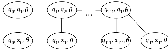
Figure 5-14: PHMM junction tree.
