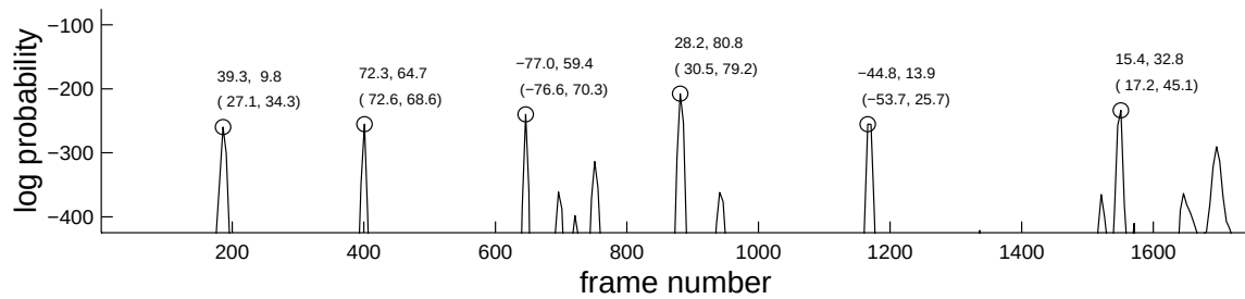
Figure 2-15: Recognition results are shown by the log probability of the windowed sequence beginning at each frame number. The true positive sequences are labeled by the value of \theta recovered by the EM testing algorithm and the value computed by direct measurement (in parentheses).
